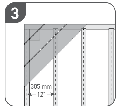
DIAGONAL INSTALLATION
